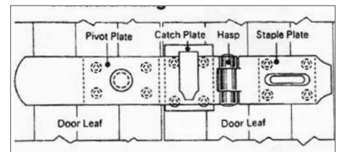
Standard fixing
